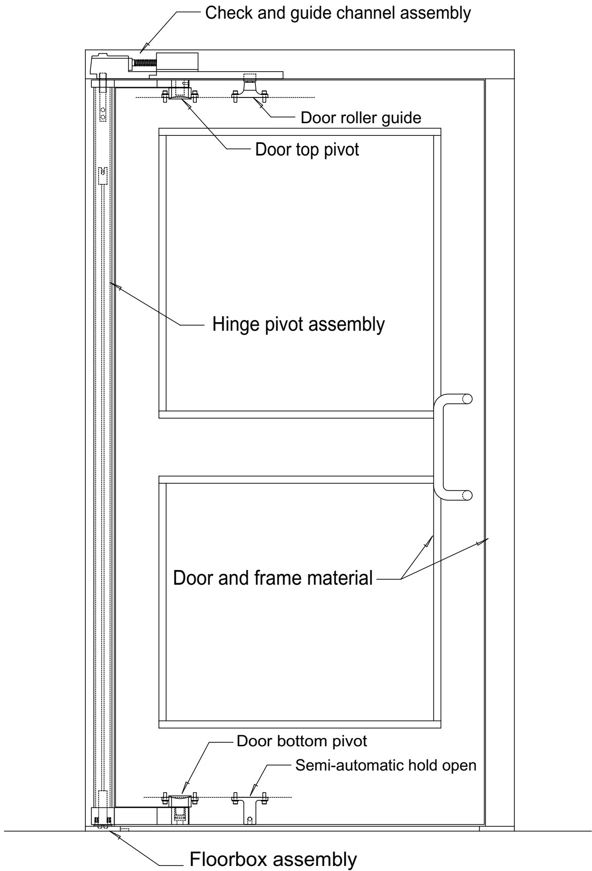
Door and frame elevation showing balanced hardware parts
