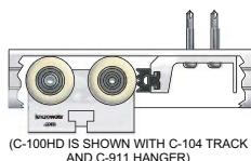
(C-100HD IS SHOWN WITH C-104 TRACK AND C-911 HANGER)
