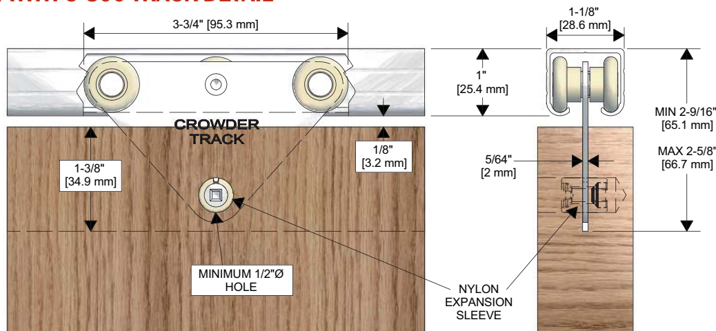
C-200 Guide or C-200B Spring Loaded Guide & C-201 Guide Channel. (See page 71 for more details).
