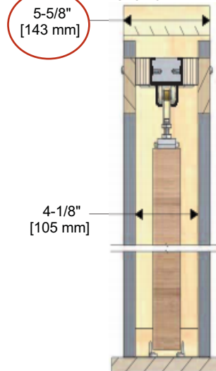
2 X 6 WALL CONSTRUCTION POCKET DOOR KIT SECTION VIEW
