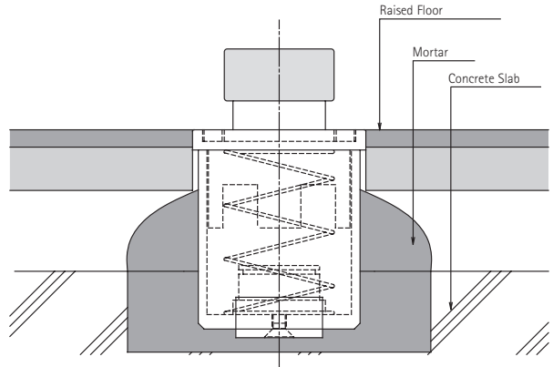
Raised Floor
